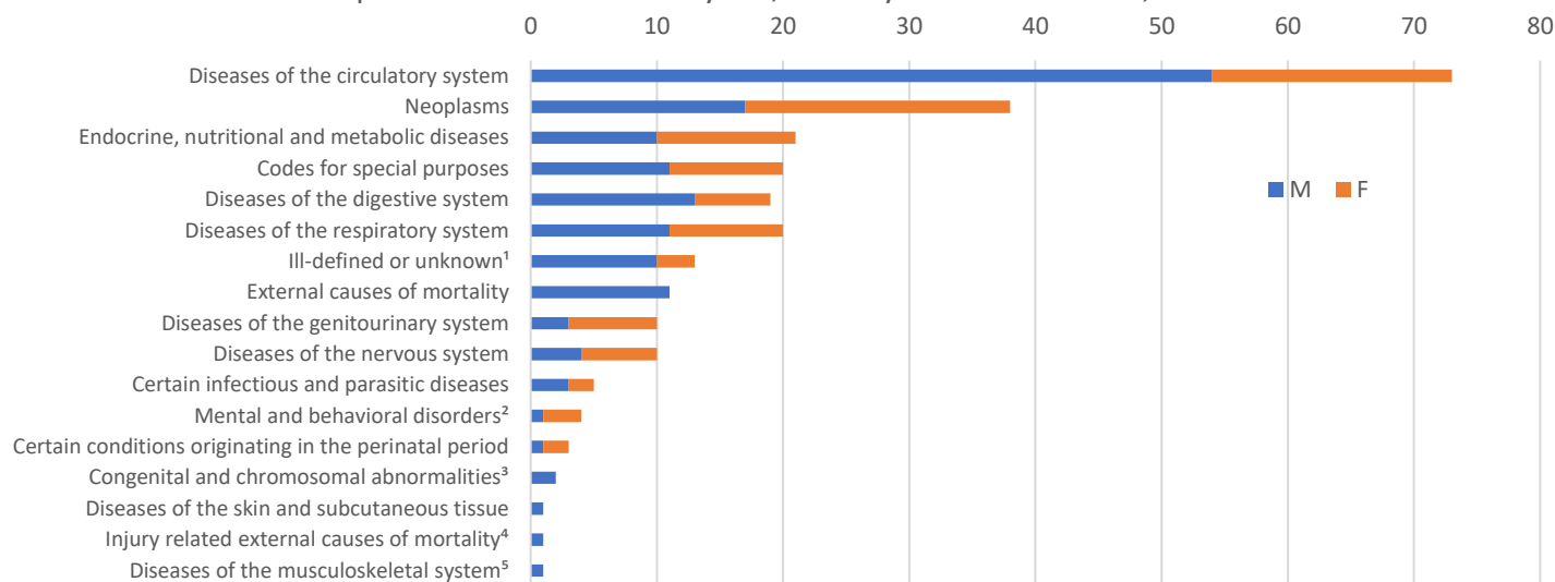
Disease-specific causes of death by sex, January 2 - November 19, 2022
